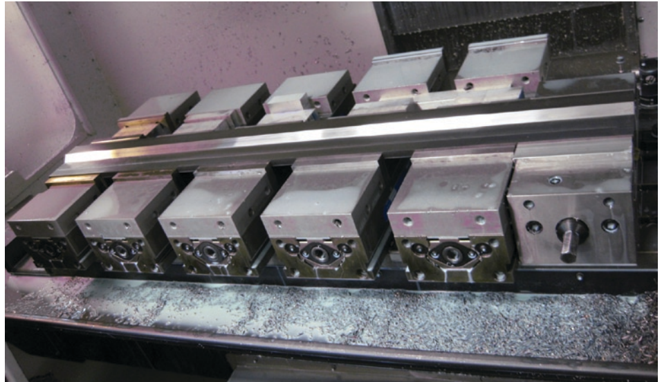
A construction component, machined from 1045 steel bar stock using a VoluMill™ toolpath.
